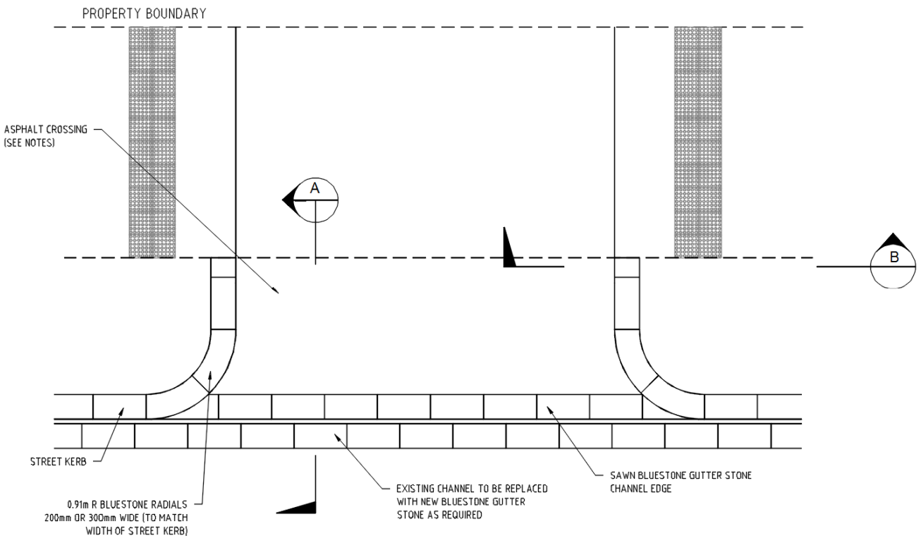
PLAN NTS
