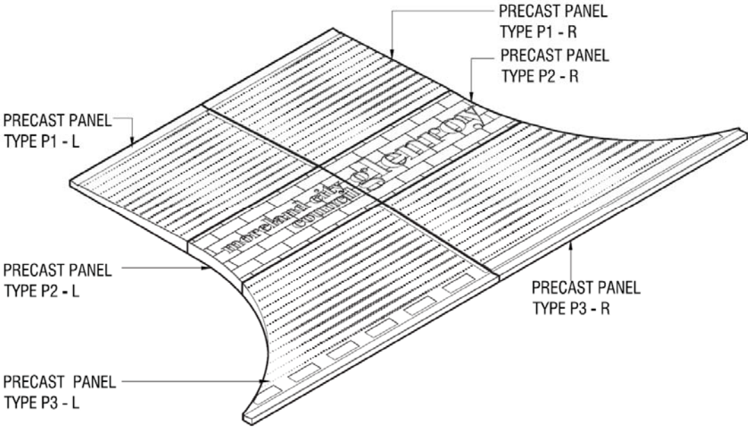
Precast concrete pedestrian crossing panels
