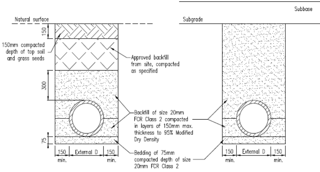
TRENCH IN NATURE STRIP
