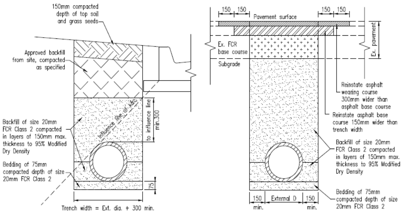
TRENCH BEHIND KERB & CHANNEL
