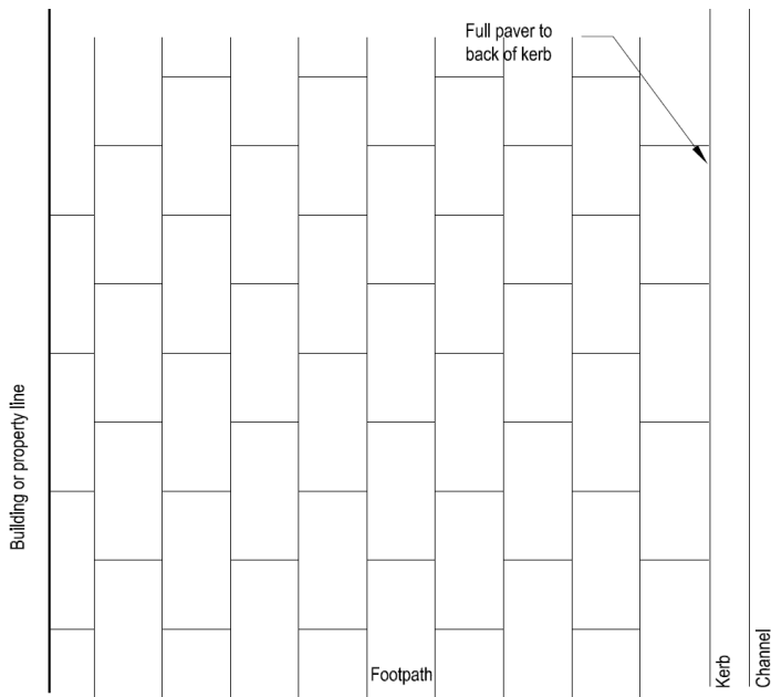
Typical Arrangement
