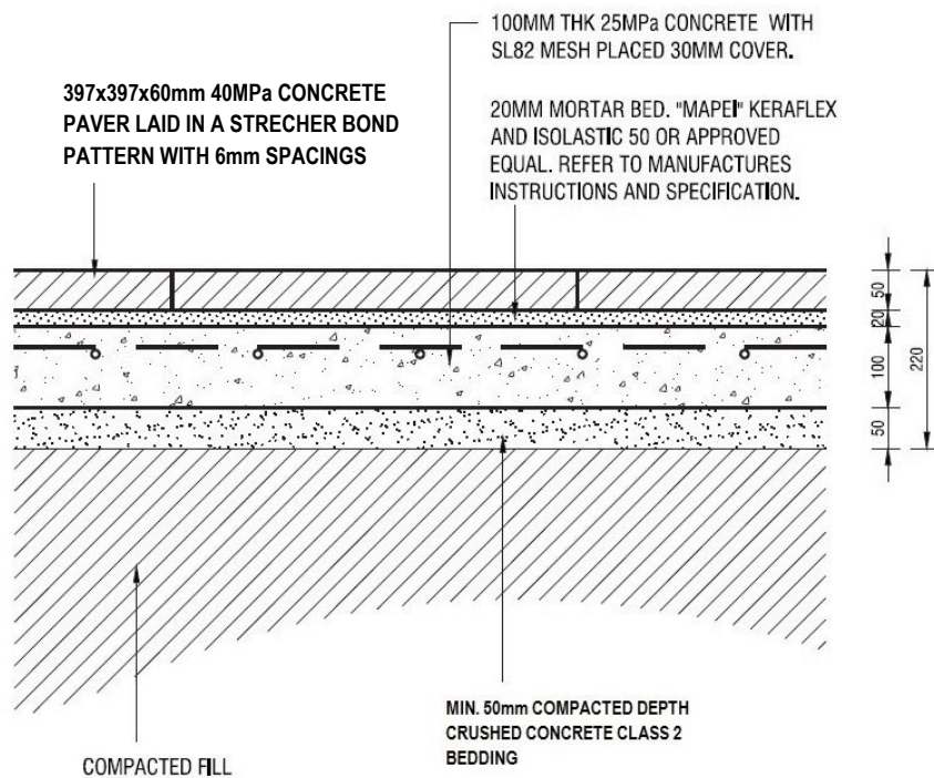
Typical Precast Concrete Paving Detail
